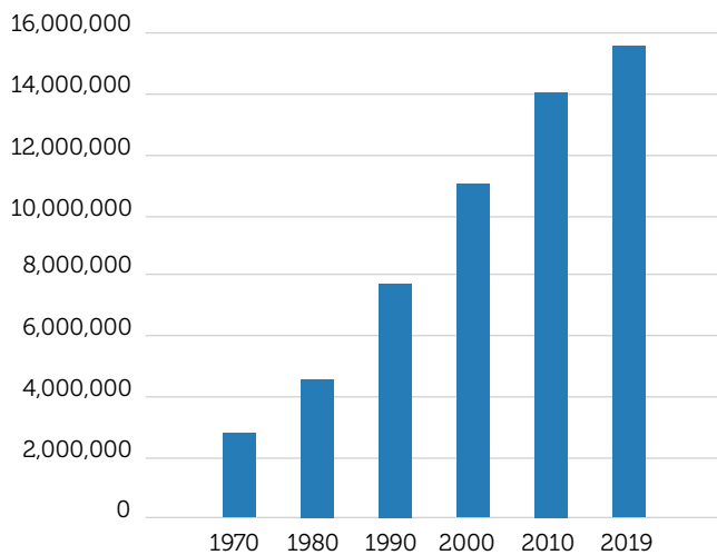
Figure 1 Latinx Population in California, 1970–2019
